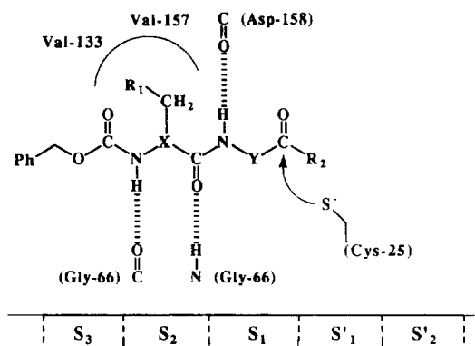
Fig 1. Schematic representation of binding of a peptidyl-methylketone inhibitor in the papain active site, as deduced from the X-ray crystallographic structure of the enzyme inhibited by Z-Phe-Gly-CH 2 -Cl [34]. In the crystal complex, the side chain of the Phe residue is out of plane with its backbone atoms and establishes hydrophobic interactions with Val-133 and Val-157 residues in the S_2 subsite of the enzyme. The catalytic thiolate of Cys-25 and atomic groups of Gly-66 and Asp-158 intervening as hydrogen-bonding partners are also reported.
