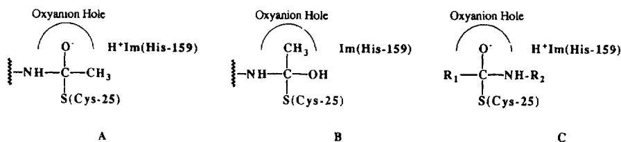
Fig 3. Postulated structures of tetrahedral intermediates for binding of 1-peptidyl-2 acetyl hydrazines 3a and 3d at the papain active site as substrate analogs (A and B) and for papain-catalyzed hydrolysis of peptidyl substrates (C). Protonation of the NH by His-159, which would facilitate cleavage of the amide linkage, can only easily intervene in the tetrahedral intermediate C.
