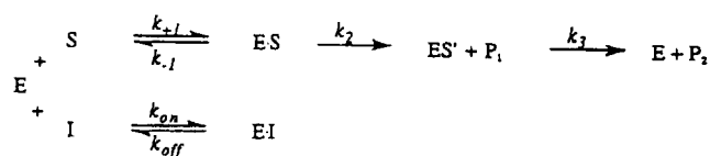
Scheme 3. Minimal reaction mechanism for the inhibition of thiol proteases by substrate analog peptidyl methylketones in the presence of substrate. The second-order rate constant for the formation of E·I is represented by k_{\text{on}} ; k_{\text{off}} is the first-order rate constant for its dissociation.
